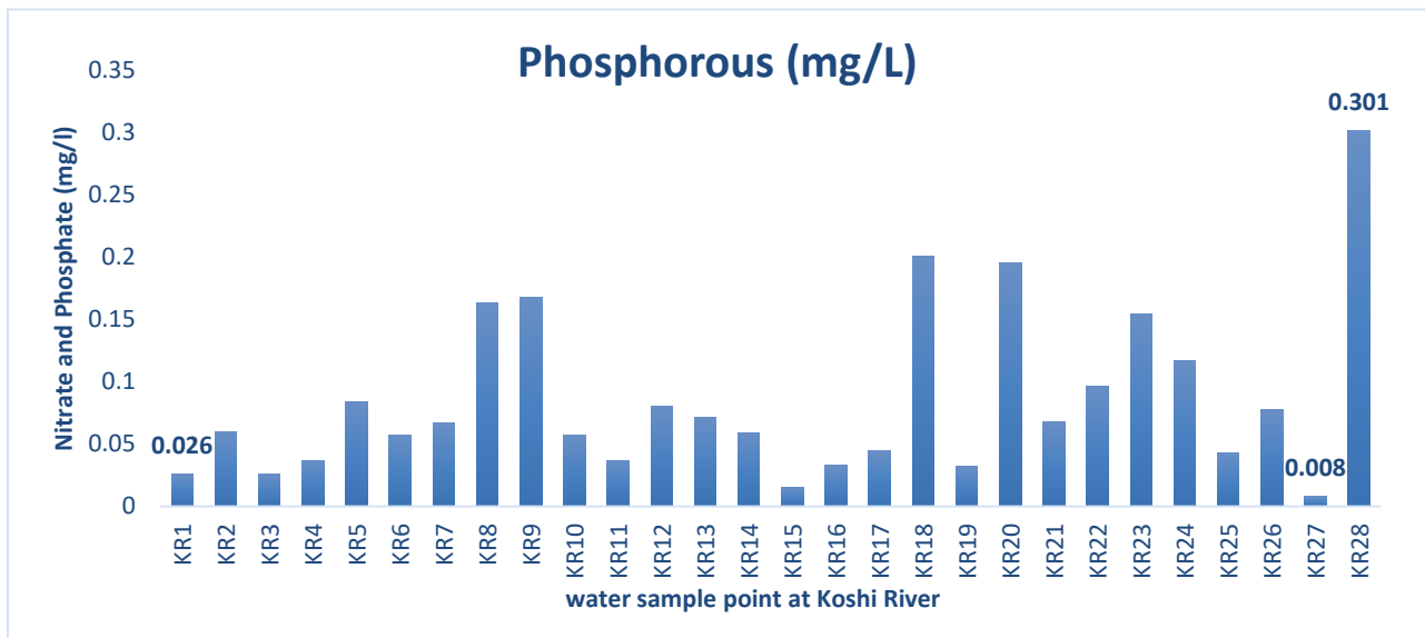
Fig: Graph illustrates the data of phosphorous sampled at 28 different sampling points of the Koshi Rivers
