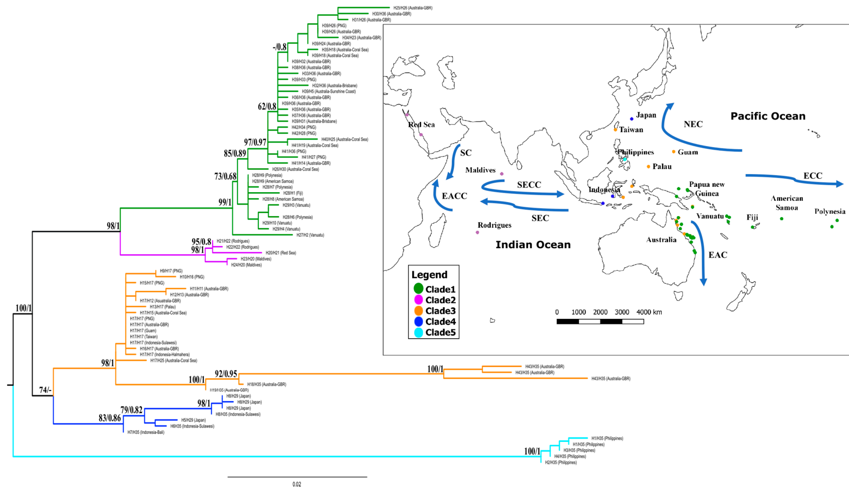
Figure 1. Midpoint rooted ML phylogenetic tree with concatenated sequences of cox3 and 28S, and a map of the sampling localities. Collapsed haplotypes for each gene ( cox3 /28S), with localities shown on root tips (refer to Supplemental S1). Ultrafast bootstrap values (UBV) above 60 and posterior probabilities (PP) above 0.60 are shown (UBV/PP). Main currents: SC = Somali current, EACC = East African coastal current, SECC = South Equatorial counter current, SEC = South Equatorial current, NEC = North Equatorial current, ECC = Equatorial counter current and EAC = East Australian current.
