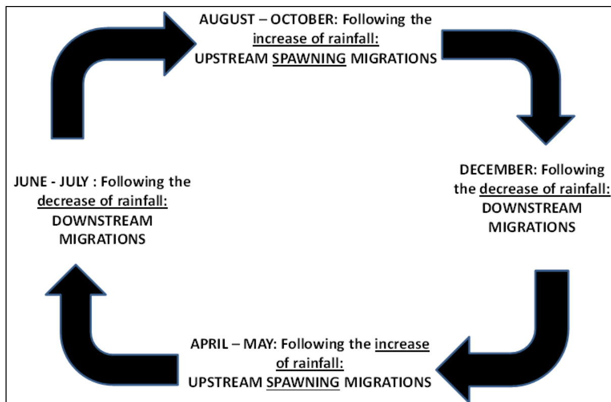
Fig 4: Synthesized migrations diagram of C. gariepinus in Lake Edward watershed, Albertine Rift Valley
